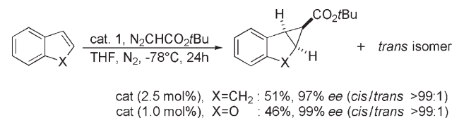
Scheme 2. Asymmetric cyclopropanation of cyclic olefins.
